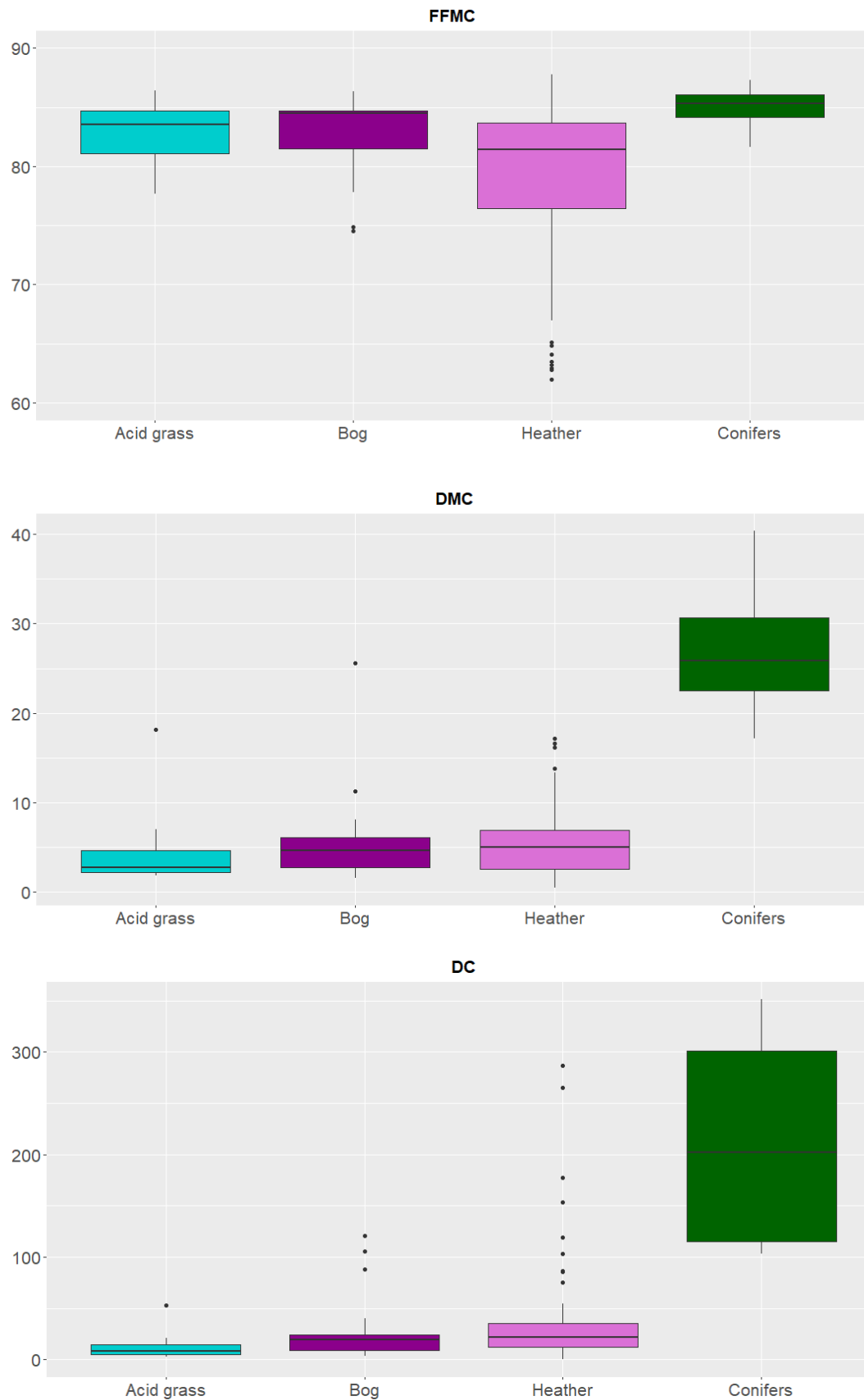
Figure 8a. Boxplots of CFWIS fuel moisture codes per dominant fuel types of fires that occurred in Scotland in the 2013-2019 period.
