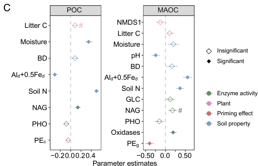
Fig. 3. Effects of abiotic and biotic factors on soil POC and mineral-associated organic carbon (MAOC). (A) correlation of soil C components with the predictors. (B) the relative importance of the plant, enzyme, priming effect, and soil properties. (C) average parameter estimates of model predictors, and associated SE. The R^2 of the averaged model and the P value are shown as * P < 0.1 ; ** P < 0.05 ; *** P < 0.01 ; **** P < 0.001 . NMDS1, the first axis of NMDS, shows the differences in plant functional composition; Al d + 0.5Fe d , weight-normalized contents of Fe d and Al d ; GLC, \beta -glucosidase; NAG, N-acetyl glucosaminidase; PHO, phosphatase; PE g , glucose-induced priming effect; PE c , cellulose-induced priming effect.
