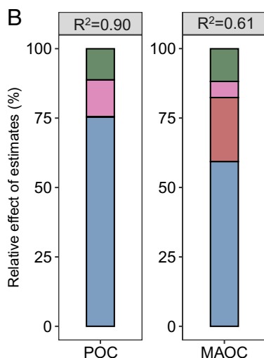
Fig. 3. Effects of abiotic and biotic factors on soil POC and mineral-associated organic carbon (MAOC). (A) correlation of soil C components with the predictors. (B) the relative importance of the plant, enzyme, priming effect, and soil properties. (C) average parameter estimates of model predictors, and associated SE. The R^2 of the averaged model and the P value are shown as * P < 0.1 ; ** P < 0.05 ; *** P < 0.01 ; **** P < 0.001 . NMDS1, the first axis of NMDS, shows the differences in plant functional composition; Al d + 0.5Fe d , weight-normalized contents of Fe d and Al d ; GLC, \beta -glucosidase; NAG, N-acetyl glucosaminidase; PHO, phosphatase; PE g , glucose-induced priming effect; PE c , cellulose-induced priming effect.
