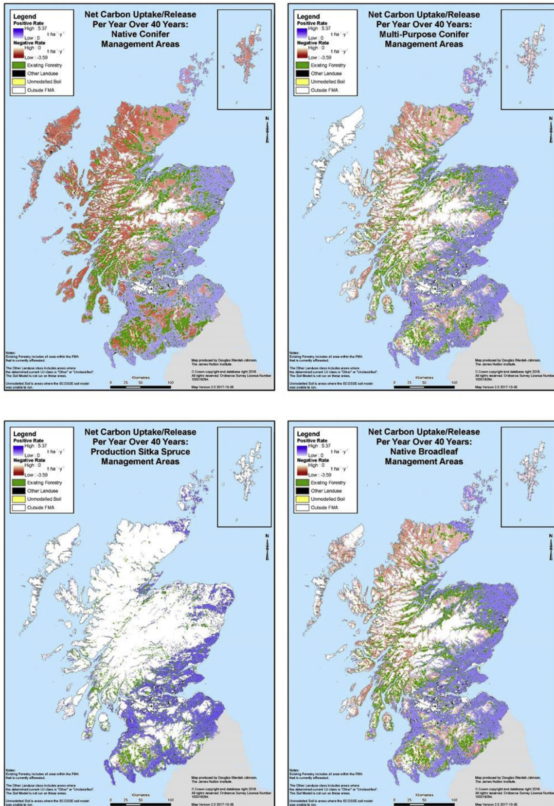
Fig. 2. Maps of carbon accumulation or loss characteristics for selected sub-FMA OPP areas.
